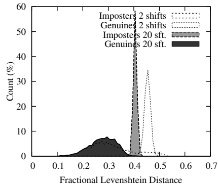
Fig. 5. Impact of max. LD shifts on Ma 's score distributions ( CASIA dataset).
