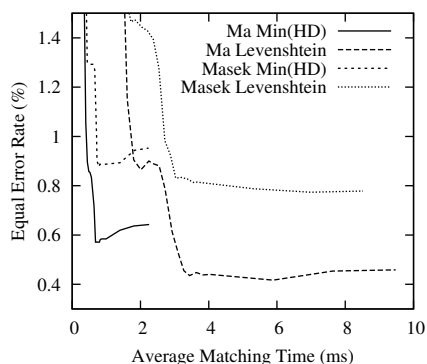
Fig. 7. Time-EER tradeoff for HD and LD on CASIA dataset.
