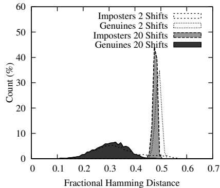
Fig. 4. Impact of max. HD shifts on Ma 's score distributions ( CASIA dataset).
